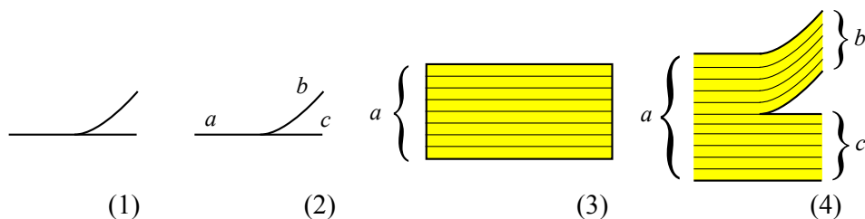
FIGURE 13. A switch (1), the switch condition requires that a = b + c (2), to construct a foliation, replace every branch with weight a with a square of width a (3), every switch creates a singular point (4).
