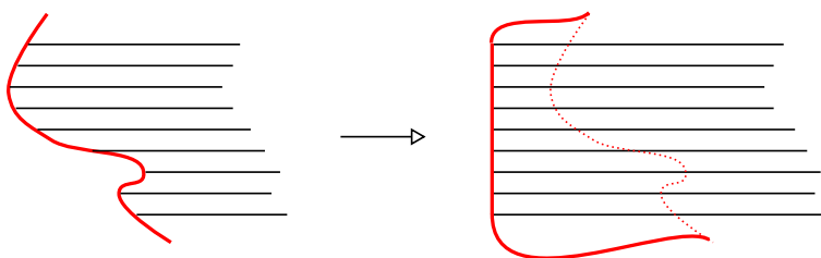
FIGURE 10. We can enlarge D so that \alpha \subset \partial D intersects \phi into lines orthogonal to the leaves.
