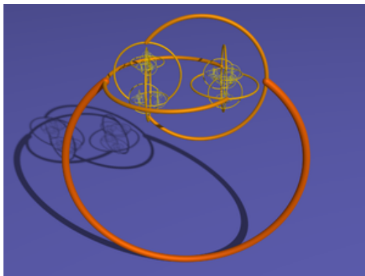
FIGURE 1. The Alexander horned sphere is a subset of \mathbb{R}^3 homeomorphic to the 2-sphere S^2 . It divides \mathbb{R}^3 into two connected components, none of which is homeomorphic to an open ball. It was constructed by Alexander as a counterexample to a natural three-dimensional generalization of Jordan's curve theorem. The natural generalization would be the following: does every 2-sphere in \mathbb{R}^3 bound a ball? If the 2-sphere is only topological, the answer is negative as this counterexample shows. If the sphere is a differentiable submanifold, the answer is however positive as proved by Alexander himself.
