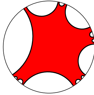
FIGURE 18. The universal covering of \Sigma is isometric to the interior of a polyhedron without vertices in \mathbb{H}^2 .
