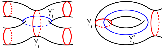
FIGURE 9. Choose for any component \gamma_i of a pants decomposition \mu a curve \gamma'_i that intersect \gamma_i in one or two points and is disjoint from the other components. There are two cases to consider, depending on whether the two pairs-of-pants adjacent to \gamma_i are distinct (left) or not (right).
