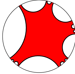
FIGURE 1. An intersection of (possibly infinitely many) half-planes. The universal cover of a hyperbolic surface with boundary is isometric to such an object.
