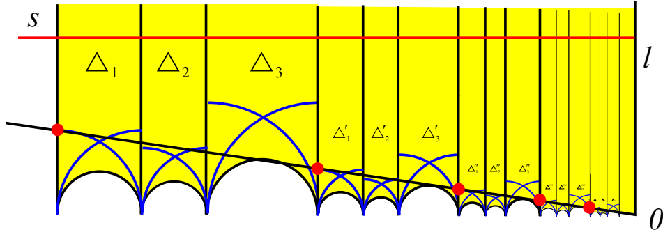
FIGURE 19. When d_1 + \dots + d_h \neq 0 , the isometry \varphi sending \Delta_1 to \Delta'_1 is hyperbolic, with some axis l which (up to translations) has endpoints 0 and \infty . Hence \varphi(z) = e^d z and the triangulation develops towards l as shown here.
