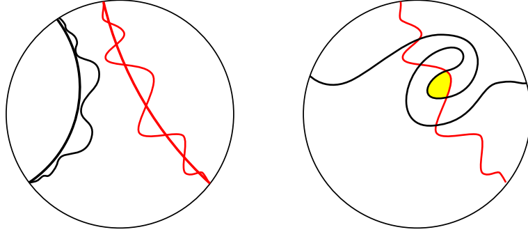
FIGURE 14. The lifts of \gamma_i and \bar{\gamma}_i have distance bounded by R and hence have the same endpoints (left). Two curves that intersect in more than one point form a bigon (right).
