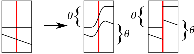
FIGURE 7. A geodesic \bar{\eta} in h_\theta^\gamma is a geodesic outside the annulus and deviates on the left by an angle \theta when crossing it (center) since h_\theta^\gamma is obtained by twisting a hyperbolic metric (left). We may simplify the picture by describing \bar{\eta} as a broken geodesic line (right).
