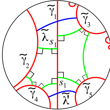
FIGURE 12. If we pick \lambda' instead of \lambda we find a segment of the same length s_1 , since the two right-angled hexagons shown are isometric.
