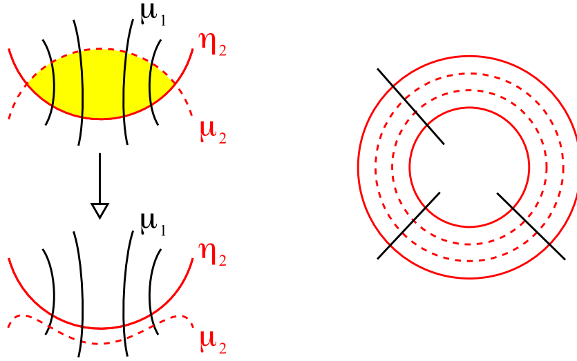
FIGURE 16. A bigon between \mu_2 and \eta_2 intersects \mu_1 into vertical arcs and can be removed via an ambient isotopy that preserves the support of \mu_1 (left). Per ogni tipo di omotopia esistono k curve in \mu_2 e k in \eta_2 e tutte queste intersecano \mu_1 in archi come in figura (destra).
