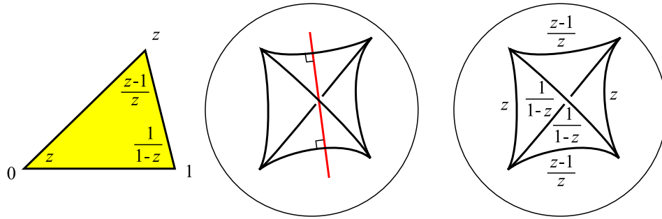
FIGURE 2. At each ideal vertex we have a euclidean triangle defined up to similarities: each vertex of the triangle has a well-defined complex angle (left). A pair of opposite edges in the ideal tetrahedron has an axis orthogonal to both which is a symmetry axis for the tetrahedron (center). We can assign the complex angles directly to the edges of the tetrahedron (right). The argument is the dihedral angle of the edge.
