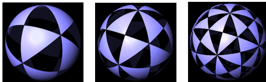
FIGURE 5. The tessellations (2, 3, 3) , (2, 3, 4) and (2, 3, 5) of the sphere.
