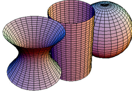
FIGURE 3. Three surfaces in space (hyperboloid of one sheet, cylinder, sphere) whose gaussian curvature is respectively negative, null, and positive at each point. The curvature on the sphere is constant, while the curvature on the hyperboloid varies: as we will see, a complete surface in \mathbb{R}^3 cannot have constant negative curvature.
