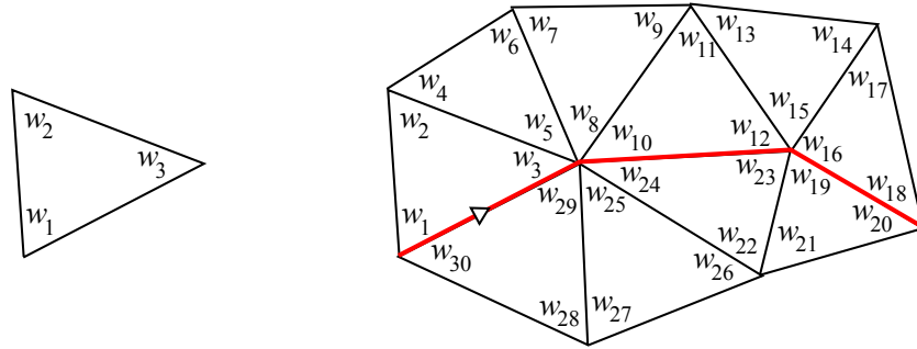
FIGURE 5. Every boundary torus Y \subset \partial N is triangulated. Each triangle has a euclidean structure well-defined up to similarities and inherits three complex moduli w_1, w_2, w_3 at its vertices (left). At every vertex of the triangulation, the product of the adjacent moduli is 1, for instance here w_{12}w_{15}w_{16}w_{19}w_{23} = 1 . The red path contributes to \mu as -w_{30}w_{29}w_{25}w_{24}w_{23}w_{19}w_{20} (right).
