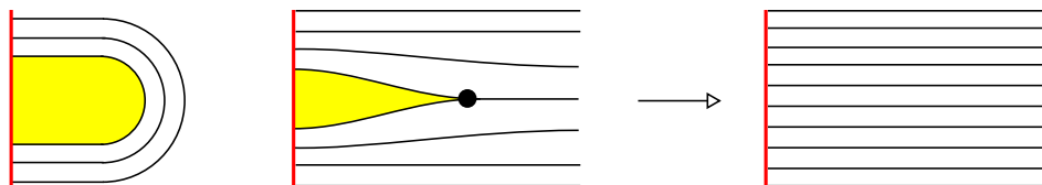
FIGURE 11. There are no complementary bigons as in the left picture. A complementary triangle as in the right picture can be eliminated by gluing together two sides of it. If the sides have different lengths, we enlarge the disc as in Fig. 10 to get sides of the same length.
