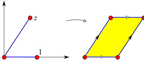
FIGURE 2. The flat metric on the torus T determined by z \in H^2 may be constructed by identifying the opposite sides of the parallelogram with vertices 0, 1, z, z + 1 . The lattice \Gamma is generated by 1 and z and the parallelogram is a fundamental domain.
