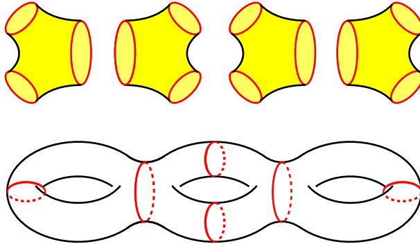
FIGURE 7. Every surface of finite type with \chi < 0 decomposes into pair-of-pants. We show here a decomposition of S_3 .
