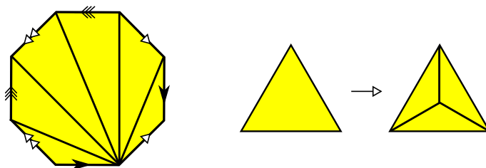
FIGURE 15. The standard representation of S_g by identifying the edges of a 4g -gon has only one vertex; if we triangulate the 4g -gon we get an ideal triangulation for S_{g,0,1} (left). A move that modifies a triangulation by adding a new vertex (right).
