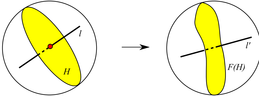
FIGURE 4. Let l and H be a line and an orthogonal hyperplane. The orthogonal projection of H onto l is obviously a point l \cap H ; the pseudo-isometry F mildly distorts this picture: the image F(H) projects to a bounded segment in l' .
