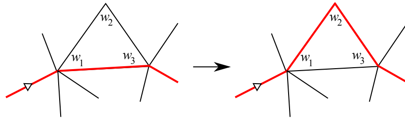
FIGURE 6. This move for \gamma does not affect \mu(\gamma) .
