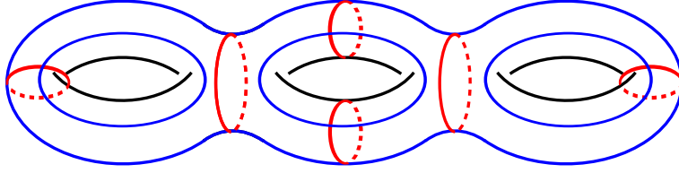
FIGURE 10. A frame for Fenchel-Nielsen coordinates consists of a (red) pants decomposition \mu and a (blue) transverse multicurve \eta that cuts each pants into two hexagons. The number of components of \mu is 3g - 3 , that of \eta can vary.
