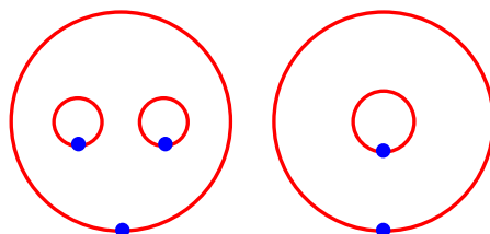
FIGURE 16. Identify each pant and annulus with one of these two fixed models.
