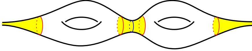
FIGURE 2. The thick-thin decomposition of a complete hyperbolic surface: the thin part (yellow) consists of truncated cusps and neighborhoods of short geodesics (blue).
