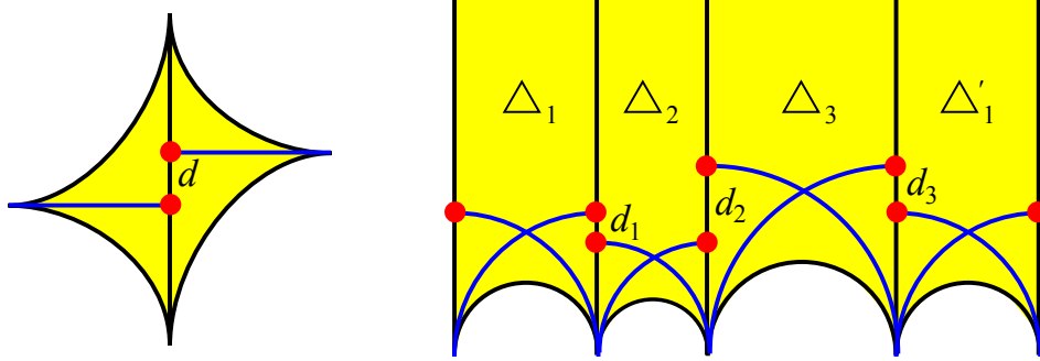
FIGURE 17. The shear is the signed distance d between two midpoints after the isometric gluing. By convention the sign is positive d > 0 if the points are as shown here (left). We develop a triangulation around a puncture v : here h = 3 (right).
