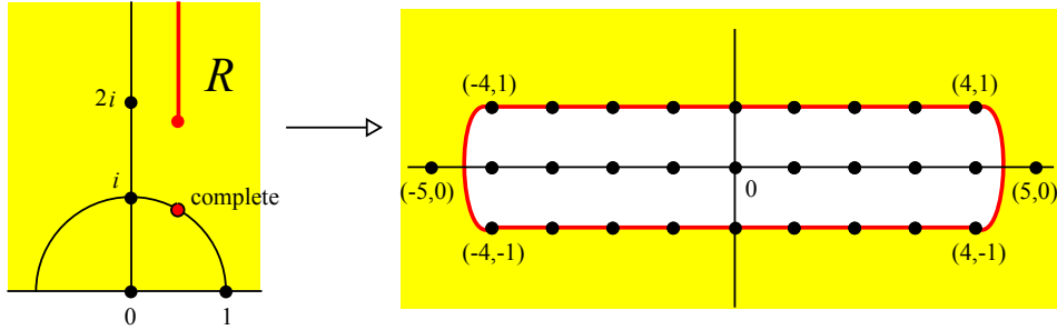
FIGURE 11. Every w \in R determines a hyperbolic structure for M (left). The Dehn filling generalized invariants map R onto a neighborhood of \infty (right).
