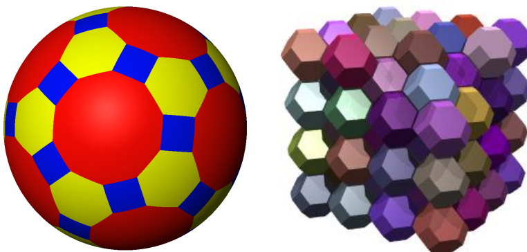
FIGURE 2. A tessellation of S^2 into squares, hexagons, and decagons, and a tassellation of \mathbb{R}^3 into truncated octahedra.
