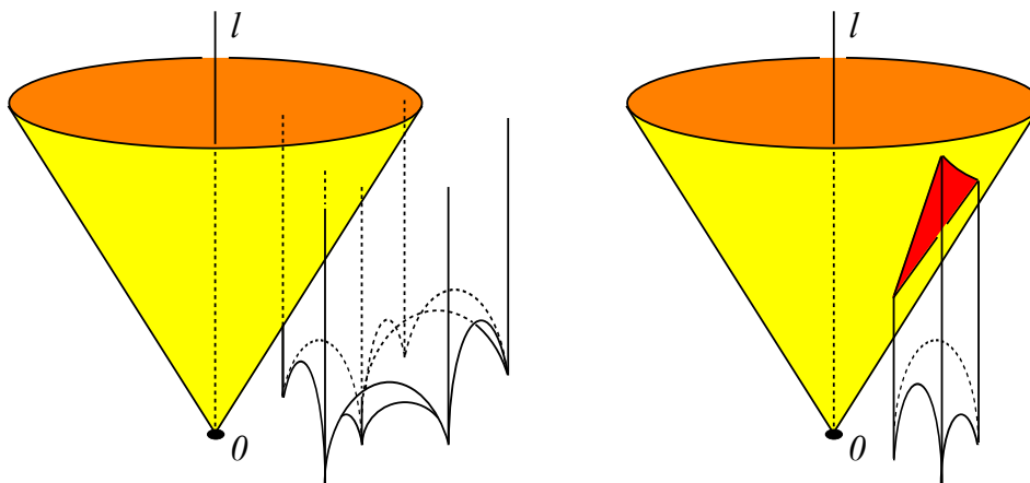
FIGURE 10. For sufficiently small R > 0 the cone neighborhood N_R(l) of l does not intersect the lower faces of \tilde{\Delta}_{i_1}, \dots, \tilde{\Delta}_{i_h} (left). These tetrahedra intersect \partial N_R(l) into triangles that glue up to determine a torus T_R in N(\Sigma) (right).
