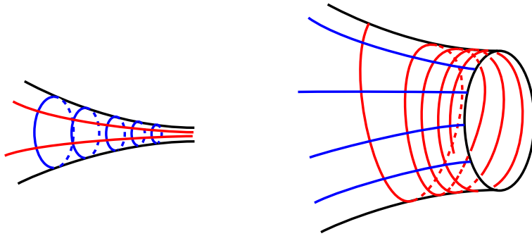
FIGURE 21. Near an ideal vertex v , horocycles (in blue) and edges of the triangulation (in red) are mutually orthogonal. They behave much differently in presence of a cusp (left) or of a geodesic boundary (right): in a cusp, horocycles form parallel circles and edges point toward the cusp; near a geodesic boundary, the horocycle point orthogonally toward the boundary and the edges spin and wind around it indefinitely.
