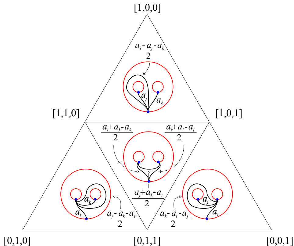
FIGURE 17. The portion of train track determined by the triple (a_i, a_j, a_k) . The triangle in \mathbb{RP}^2 with vertices [1, 0, 0] , [0, 1, 0] , [0, 0, 1] subdivides into four triangles and the shape of the train track depends on the position of P = [a_i, a_j, a_k] . When P lies in the frontier of two triangles some branch has weight zero and the different shapes actually coincide after deleting this branch.
