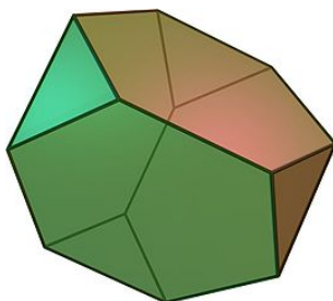
FIGURE 3. A truncated tetrahedron.
