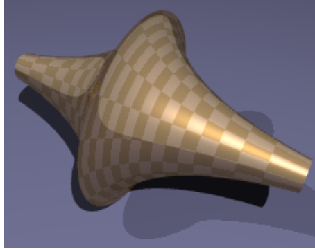
FIGURE 1. The pseudosphere is a surface in \mathbb{R}^3 isometric to the union of two truncated cusps, each with constant gaussian curvature -1 .
