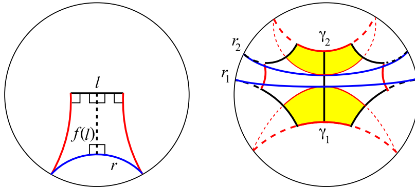
FIGURE 14. For every l there is a unique right-angled hexagons with alternate sides of length l, 0, 0 . Let f(l) be the distance between the opposite sides l and r (left). We draw a geodesic pair-of-pants as the union of two isometric hexagons: the closed geodesics \gamma_1 and \gamma_2 have disjoint f(l_1) and f(l_2) -neighborhoods, colored here in yellow (right).
