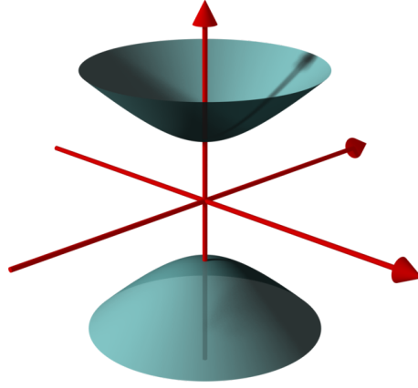
FIGURE 1. The hyperboloid with two sheets defined by the equation \langle x, x \rangle = -1 . The model I^n is the upper connected component.
