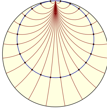
FIGURE 11. A horocycle in \mathbb{H}^2 centered in p \in \partial\mathbb{H}^2 is a circle tangent to p . It is orthogonal to all the lines exiting from p .
