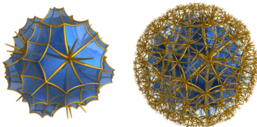
FIGURE 13. The tessellation of \mathbb{H}^3 into regular cubes with dihedral angle \theta = \frac{2\pi}{5} in the disc model.
