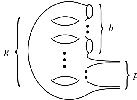
FIGURE 2. The finite type surface S_{g,b,p} .
