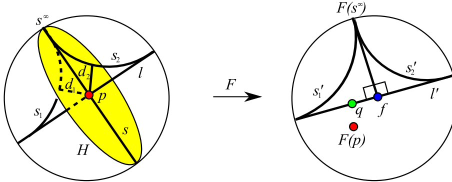
FIGURE 5. The lines s_1 and s_2 have fixed distance d_1 = d_2 = \cosh^{-1} \sqrt{2} from p . The lines l' , s'_1 , and s'_2 approximate up to an error R the images of l , s_1 , and s_2 . The projection q of F(p) on l' is hence R -close to F(p) , which is in turn (C_1 d) -close to the lines s'_i . Therefore q is (C_1 d + 2R) -close to both s'_1 and s'_2 . This easily implies that f is (C_1 d + 2R) -close to q .
