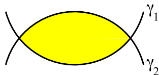
FIGURE 12. Two curves \gamma_1 and \gamma_2 are in minimal position if and only if they do not create bigons.
