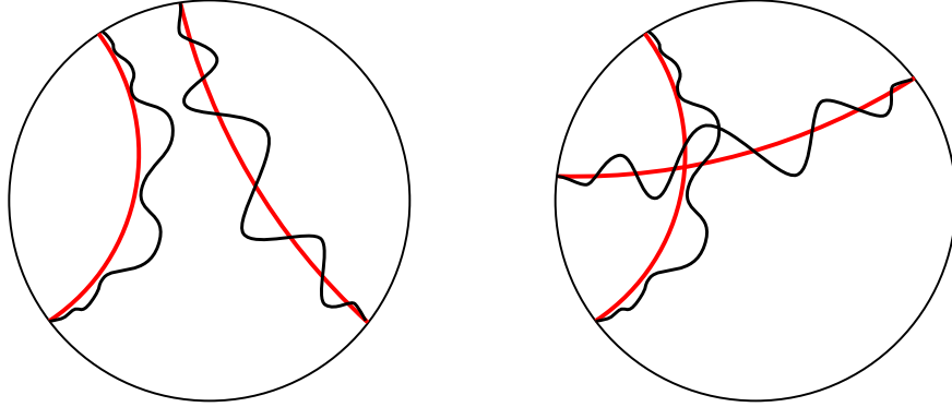
FIGURE 11. The lifts of \gamma (black arcs) and its geodesic representative (red lines) have the same endpoints in \partial\mathbb{H}^n (left). If two lines intersect, the corresponding arcs do (right).
