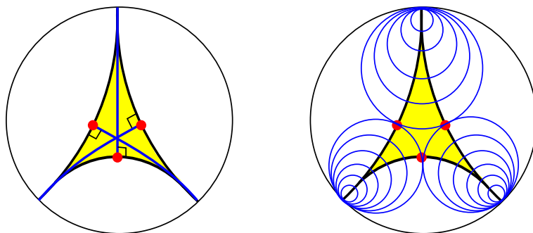
FIGURE 16. On an ideal triangle every edge has a unique perpendicular which intersects the opposite vertex. The intersection of the edge and its perpendicular is the midpoint of the edge and the three perpendiculars intersect in a point called barycenter (left). There is a unique configuration of three pairwise tangent horocycles centered at the vertices; their tangency points are the midpoints of the edges (right).
