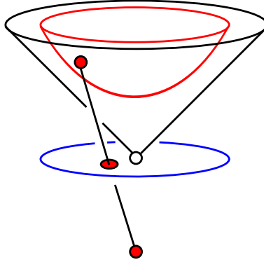
FIGURE 2. The projection on P = (0, \dots, 0, -1) induces a bijection between I^n and D^n .
