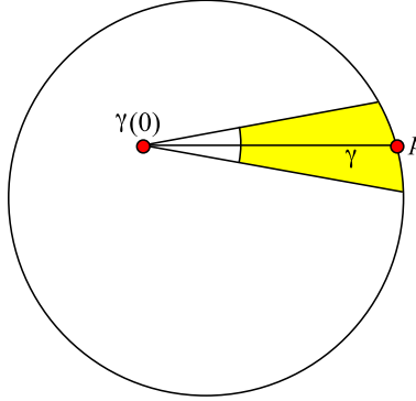
FIGURE 9. An open neighborhood U(\gamma, V, r) of p \in \partial\mathbb{H}^n (in yellow).
