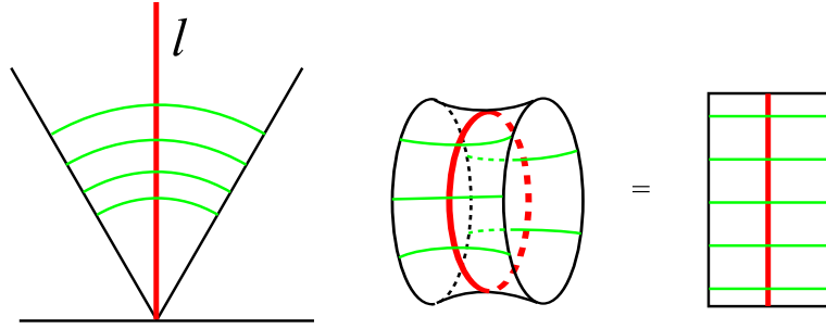
FIGURE 4. A R -annulus around a geodesic \gamma is the quotient of a R -neighborhood of a line l by a hyperbolic transformation. The orthogonal (green) geodesic segments are parametrized by arc-length as [-R, R] , hence the R -annulus is naturally parametrized as \gamma \times [-R, R] .
