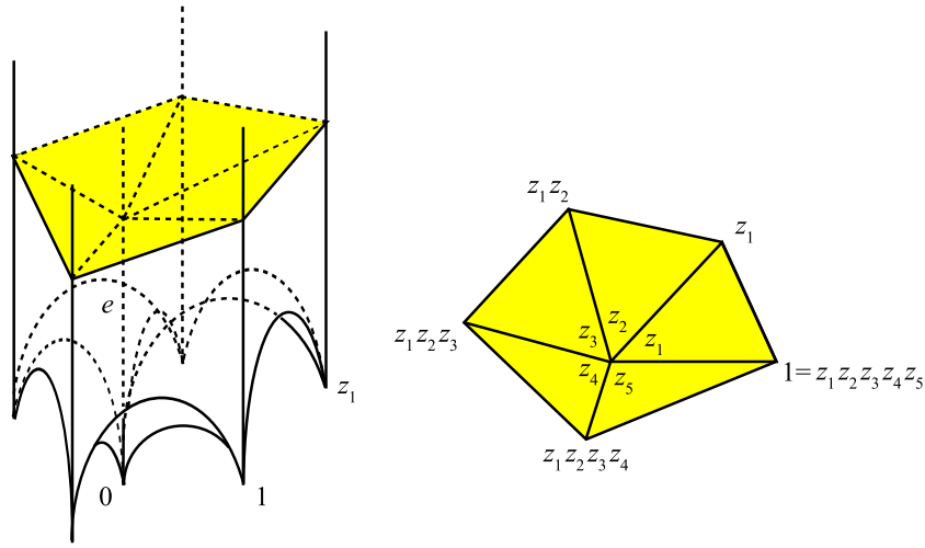
FIGURE 4. If we manage to glue all the tetrahedra incident to an edge e inside \mathbb{H}^3 as shown, the hyperbolic structure is defined also in e (left). Let z_1, \dots, z_h be the complex moduli assigned to the sides of the h incident tetrahedra (here h = 5 ). We can glue everything in \mathbb{H}^3 if and only if z_1 \cdots z_h = 1 and the arguments sum to 2\pi (right).
