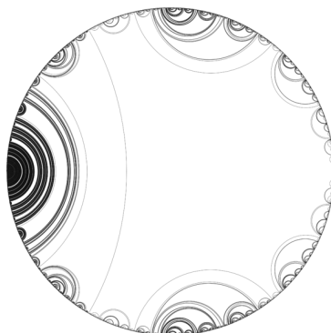
FIGURE 1. A geodesic lamination in \mathbb{H}^2 .
