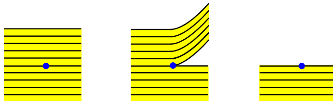
FIGURE 3. An interior, singular, and boundary point in a euclidean singular foliation.
