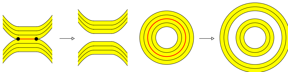
FIGURE 4. We may cut a foliation along an interior compact leaf.
