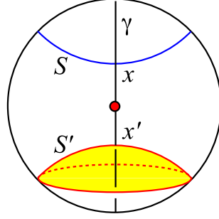
FIGURE 10. Two disjoint subspaces S, S' and a line \gamma orthogonal to both.
