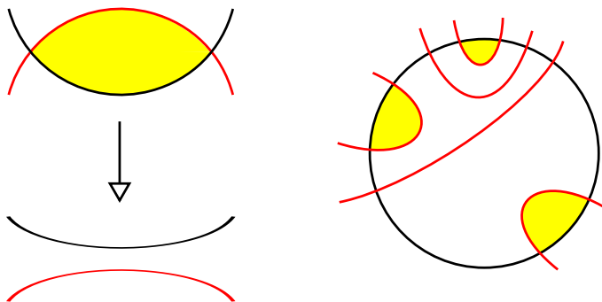
FIGURE 13. A bigon can be eliminated via homotopies (left). If \gamma_1 bounds a disc and \gamma_2 intersects \gamma_1 , there is a bigon (right).
