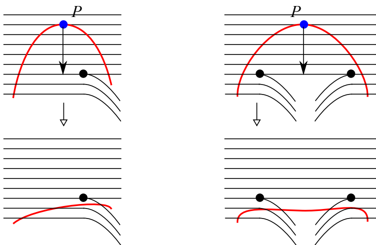
FIGURE 9. Each such configuration can be simplified.
