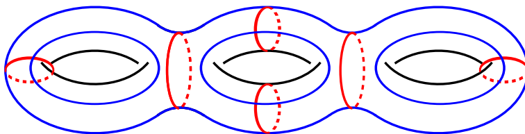
FIGURE 17. Two multicurves (blue and red) in minimal position.
