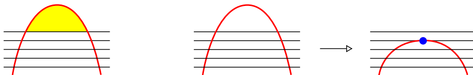
FIGURE 5. A bigon between a multicurve \mu and a foliation \phi (left) and how to eliminate it (right).
