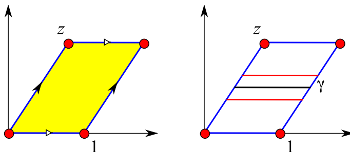
FIGURE 6. A torus with metric z (left) twisted along the curve \gamma (right).
