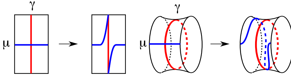
FIGURE 3. A Dehn twist along a curve \gamma maps a transverse arc \mu onto an arc which makes a complete left turn.
