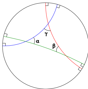
FIGURE 3. Three lines that determine a hyperbolic triangle in the Poincaré disc. The angles \alpha, \beta e \gamma coincide with the euclidean ones.
