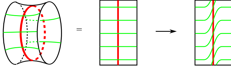
FIGURE 5. To define the earthquake we pick a diffeomorphism of the R -annulus that modifies the orthogonal segments as shown here.
