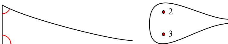
FIGURE 1. The orbifold \mathbb{H}^2/\mathbb{PGL}_2(\mathbb{Z}) has three mirrors, two of which are infinite and converge to a cusp, and two cones of angle \frac{\pi}{2} and \frac{\pi}{3} . The orbifold has area \frac{\pi}{6} . The index-two subgroup \mathbb{PSL}_2(\mathbb{Z}) < \mathbb{PGL}_2(\mathbb{Z}) that contains only orientation-preserving transformations produce the orbifold \mathbb{H}^2/\mathbb{PSL}_2(\mathbb{Z}) (right) of area \frac{\pi}{3} , obtained by mirroring the one on the left. It has a cusp and two cone points with rotational isotropy \mathbb{Z}_2 e \mathbb{Z}_3 .
