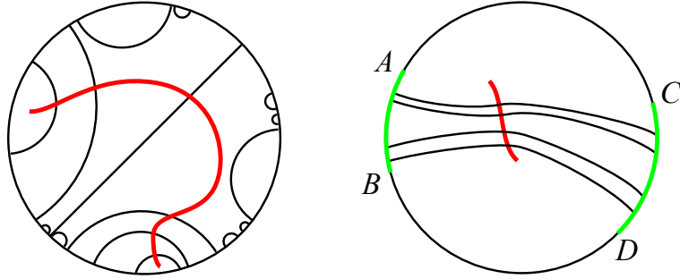
FIGURE 12. The lift \tilde{\beta} of a leaf intersects the ultraparallel lines \tilde{\mu} , each at most once: therefore it has disjoint limits as t \rightarrow \pm\infty (left). An arc crosses a first and a last leaf of \tilde{\phi} , and all other leaves it crosses have endpoints in the segments AB and CD (right).
