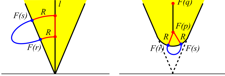
FIGURE 2. The red paths give better estimates for the distance between F(r) and F(s) . On the left: since F is C_1 -Lipschitz, the blue path has length at most C_1 d(r, s) . Its projection onto l has dilatation at most 1/\cosh R by Lemma 2.8, hence the red path in l has length at most C_1 d(r, s)/\cosh R . Therefore d(F(r), F(s)) \leq C_1 \frac{d(r, s)}{\cosh R} + 2R . On the right we get d(F(r), F(s)) \leq 2R .
