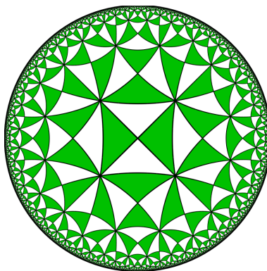
FIGURE 4. A tessellation of S^2, \mathbb{R}^2 o \mathbb{H}^2 is a subdivision of the plane into polygons. The tessellation of \mathbb{H}^2 shown here is obtained by drawing infinitely many lines in the plane. The triangles have inner angles \frac{\pi}{2}, \frac{\pi}{10}, \frac{\pi}{10} and are all isometric.
