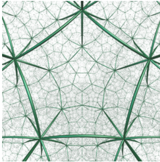
FIGURE 12. The tessellation of \mathbb{H}^3 into regular dodecahedra with dihedral angle \theta = \frac{2\pi}{5} in the disc model.
