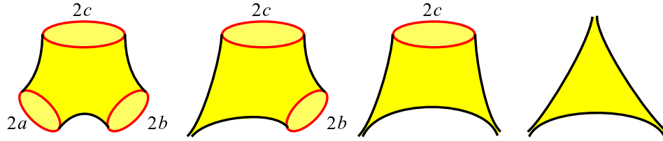
FIGURE 3. A pair-of-pants, an annulus with one puncture, a disc with two punctures, and a thrice-punctured sphere.
