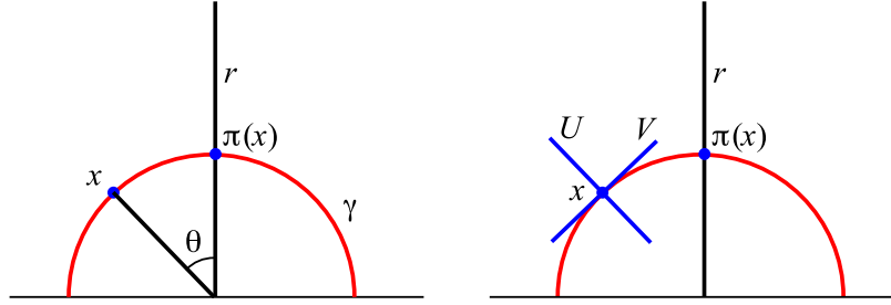
FIGURE 1. The hyperbolic cosine of the distance between x e \pi(x) is the inverse of the cosine of \theta (left). To determine the maximum dilatation we decompose the tangent space T_x (right).
