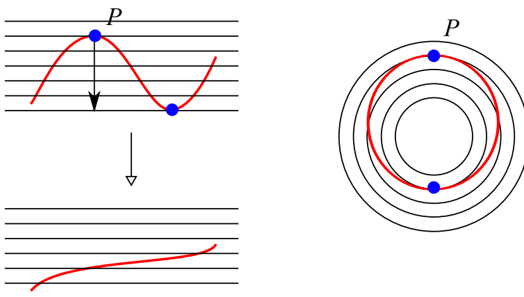
FIGURE 8. Each such configuration can be simplified. In the left picture we reduce the number of tangency points, in the right picture a component of \mu is isotopic to a leaf, hence to a boundary leaf since \phi is reduced: therefore it may be isotoped to be disjoint from \phi .
