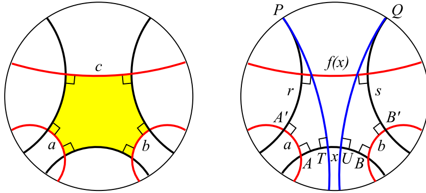
FIGURE 4. A right-angled hexagon with alternate sides of length a , b e c (left) and its construction (right), which goes as follows: take a line with two arbitrary points A and B in it (bottom black). Draw the perpendiculars from A and B (red). At distances a and b we find two points A' e B' and we draw again two perpendiculars (black) r and s , with some points at infinity P and Q . Draw the (unique) perpendiculars to the initial line pointing to P and Q (blue): they determine two points T and U . Note that AT and UB have some fixed length depending only on a and b . We can vary the parameter x = TU : if x > 0 the blue lines are ultra-parallel and there is a unique segment orthogonal to both of some length f(x) .
