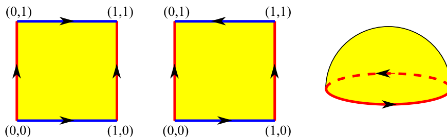
FIGURE 4. A fundamental domain in \mathbb{R}^2 for the torus (left) and the Klein bottle (center): opposite sides should be identified as indicated by the arrows. A fundamental domain in S^2 for \mathbb{R}\mathbb{P}^2 (right).
