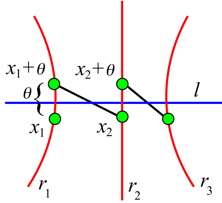
FIGURE 8. The (blue) line l is a lift of \bar{\eta} . Consider n consecutive intersections with lifts of \gamma (in red): the (n+1) -th lift is equivalent to the first via the hyperbolic transformation \tau having axis l (here n=2 ).
