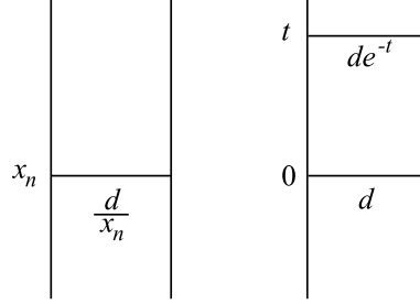
FIGURE 8. Two vertical lines in the half-space model H^n at euclidean distance d . The hyperbolic length of the horizontal segment between them at height x_n is \frac{d}{x_n} and hence tends to zero as x_n \rightarrow \infty (left). Using as a height parameter the more intrinsic hyperbolic arc-length, we see that the two vertical geodesics \gamma_1 e \gamma_2 approach at exponential rate, since d(\gamma_1(t), \gamma_2(t)) \leq de^{-t} (right).
