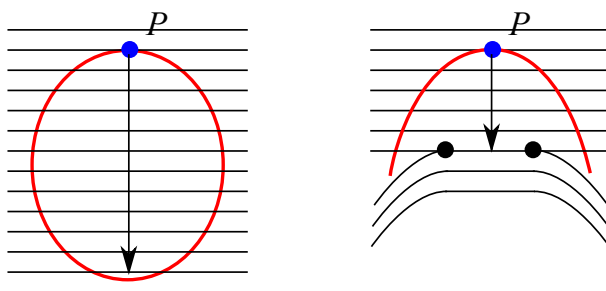
FIGURE 7. These two configurations do not arise because every component of a multicurve is homotopically non-trivial (left) and because the foliation is reduced (right).
