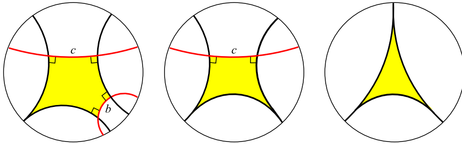
FIGURE 5. A right-angled hexagon with parameters a, b, c \geq 0 degenerates to a pentagon, quadrilateral, or triangle with ideal vertices if one, two, or three parameters are zero.
