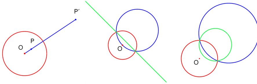
FIGURE 5. The inversion through a sphere of center O and radius r moves P to P' so that OP \times OP' = r^2 (left) and transforms a k -sphere S into a k -plane if O \in S (center) or a k -sphere if O \notin S (right).
