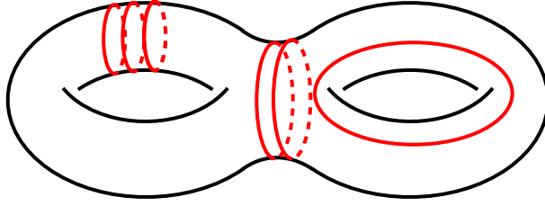
FIGURE 15. A multicurve in a surface of genus two.
