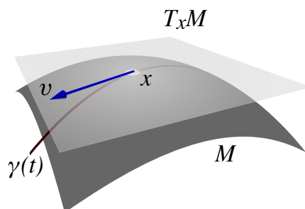
FIGURE 2. The tangent space in x may be defined as the set of all curves \gamma with \gamma(0) = x seen up to an equivalent relation that identifies two curves having (in some chart) the same tangent vector at x . This condition is chart-independent.
