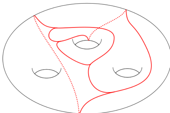
FIGURE 14. A train track on S_3 .
