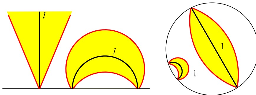
FIGURE 10. The R -neighborhood of a geodesic l in the half-plane (left) and disc (right) models.
