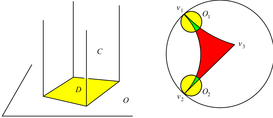
FIGURE 8. The cone C over a domain D \subset O has volume proportional to the area of D (left). If the domain is compact, the cone has finite volume: therefore an ideal polyhedron has finite volume (right).
