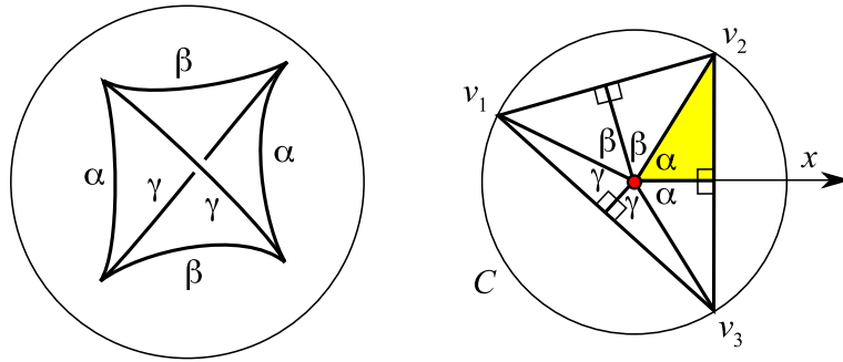
FIGURE 12. The dihedral angles \alpha, \beta, \gamma of an ideal tetrahedron. Opposite edges have the same angle and \alpha + \beta + \gamma = \pi .
