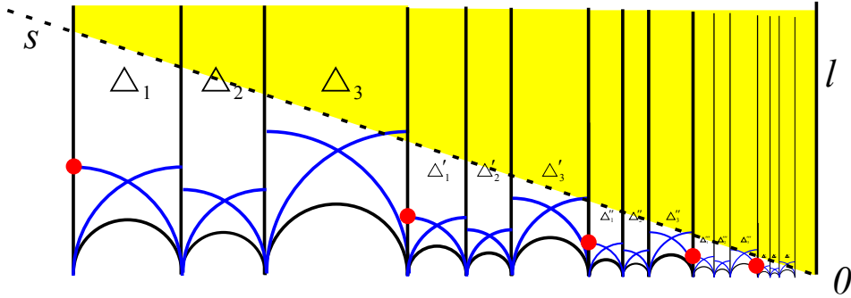
FIGURE 20. Let s be a line at distance R from l . If R is sufficiently small, the line s does not intersect the lower edges of \Delta_1, \Delta_2, \Delta_3 .
