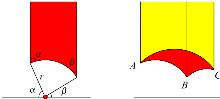
FIGURE 9. A triangle with at least an ideal vertex (left). The area of a triangle with finite vertices can be derived as the area difference of triangles with one ideal vertex (right).
