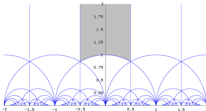
FIGURE 3. The shadowed polyhedron is a fundamental domain for \mathbb{P}\mathrm{SL}_2(\mathbb{Z}) . The translates of the fundamental domain form a tessellation.
