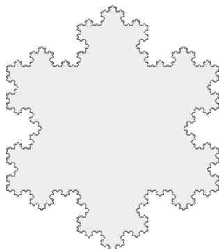
FIGURE 8. The interior of Koch snowflake is biolomorphic to an open disc.
