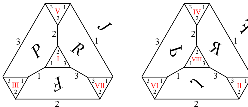
FIGURE 8. We truncate the tetrahedra and flatten their boundary. We assign a modulus z and w to them. The edge numbered i = 1, 2, 3 has modulus z_i (on the left tetrahedron) or w_i (on the right tetrahedron).
