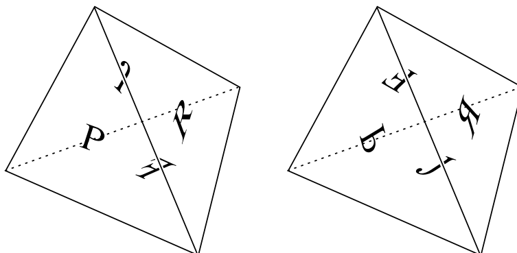
FIGURE 7. A triangulation with 2 tetrahedra. Faces with the same letter F, J, P, R are paired with a simplicial map that matches the letters.
