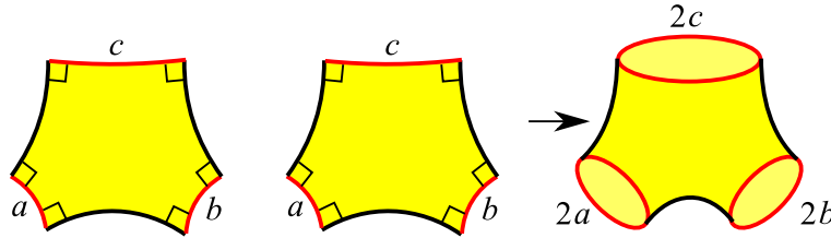
FIGURE 6. By gluing two identical right-angled hexagons along their black sides we get a hyperbolic pair-of-pants with geodesic boundary.
