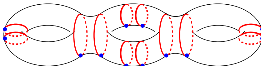
FIGURE 15. Decompose S into pants and annuli and fix a blue point in each curve.
