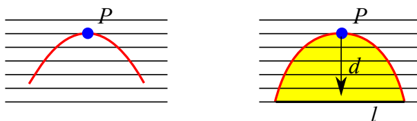
FIGURE 6. If \mu is in general position with respect to \phi , it is tangent to some leaf in finitely many points as shown here (left). A perpendicular of small length d points to some leaf l at distance d from P , which forms a bigon with \mu (right).
