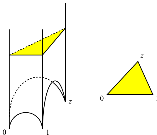
FIGURE 1. An ideal tetrahedron with three vertices in 0, 1, \infty in the half-space mode is determined by the position z \in \mathbb{C} \cup \{\infty\} of the fourth vertex. A little horosphere centered in the ideal vertex intersects the tetrahedron in a euclidean triangle uniquely determined up to similarities.
