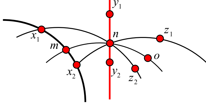
FIGURE 12. Distance between points in disjoint lines is a strictly convex function in hyperbolic space.
